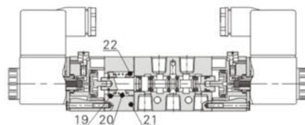
●4V430C
